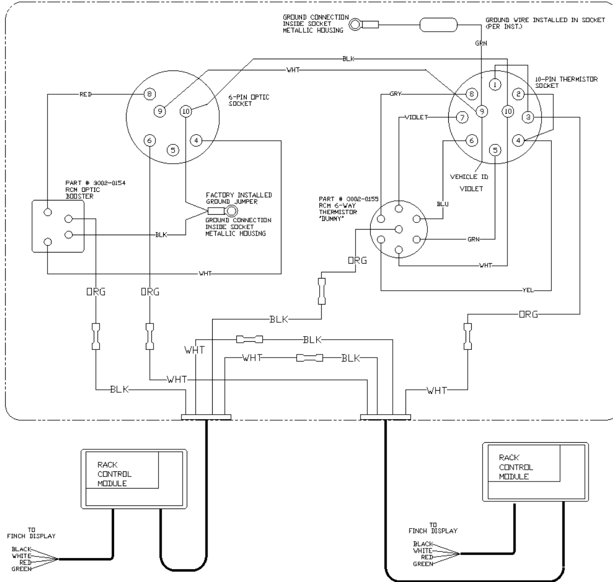
DUAL API OPTIC & THERMISTOR SOCKETS FOR RCM (USA) PART # 3002-0151
